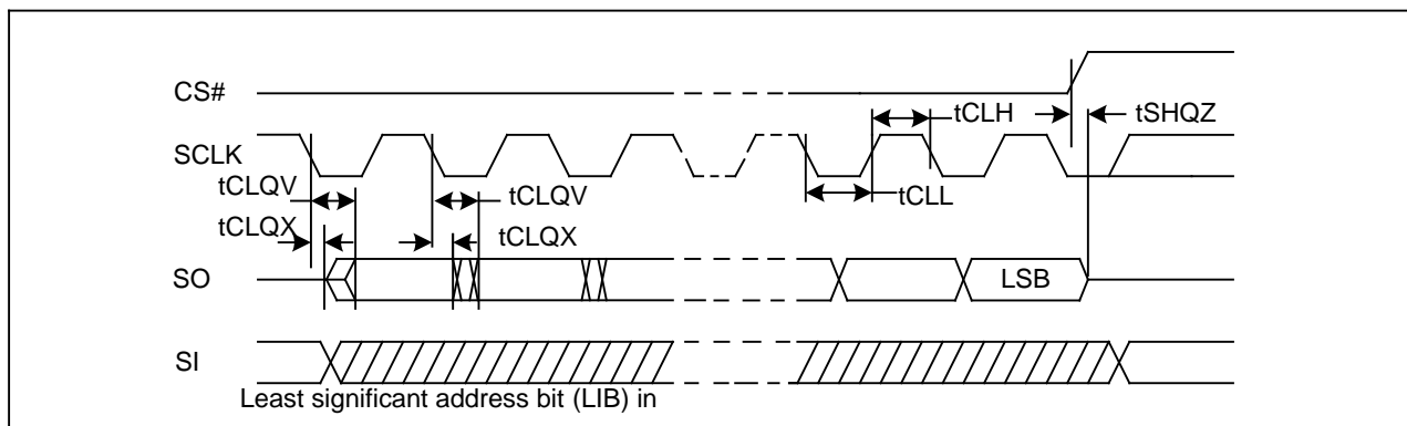
Figure36. Output Timing
