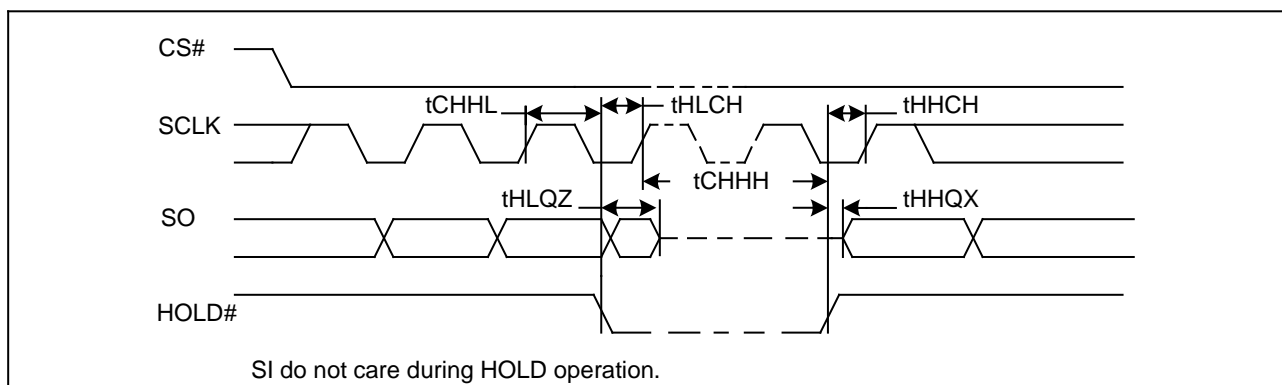
Figure37. Hold Timing
