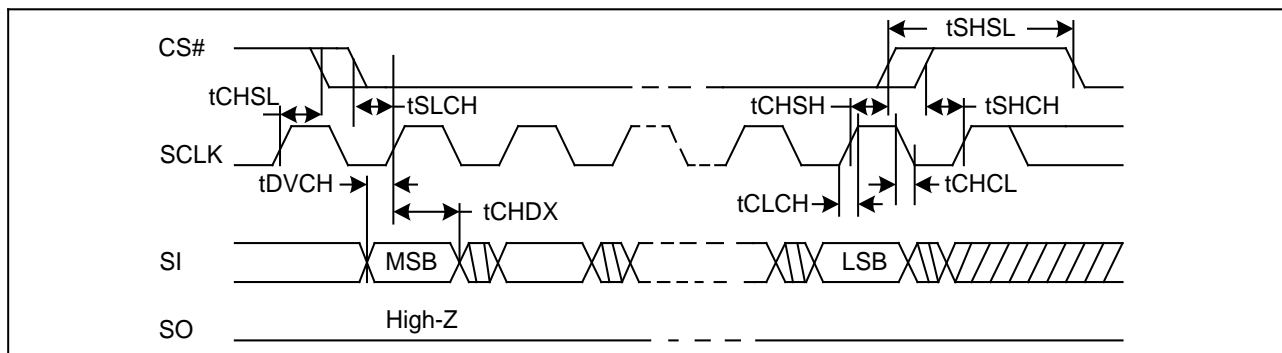
Figure35. Serial Input Timing
