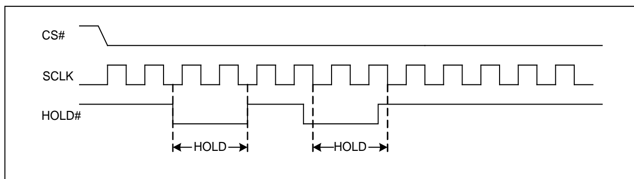
Figure1. Hold Condition
