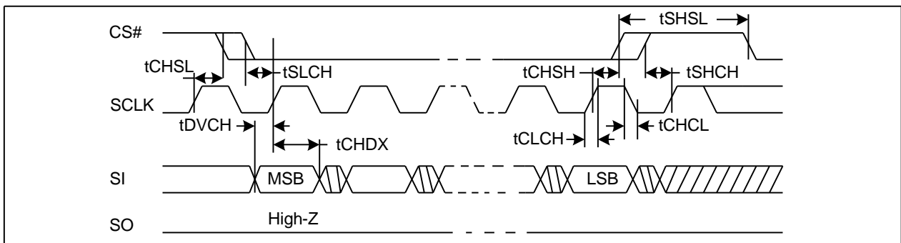
Figure26. Output Timing
