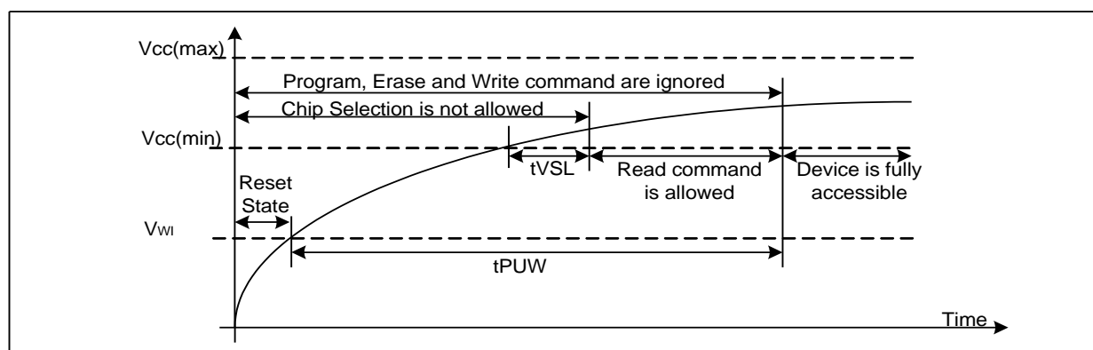
Figure23. Power on Timing Sequence
