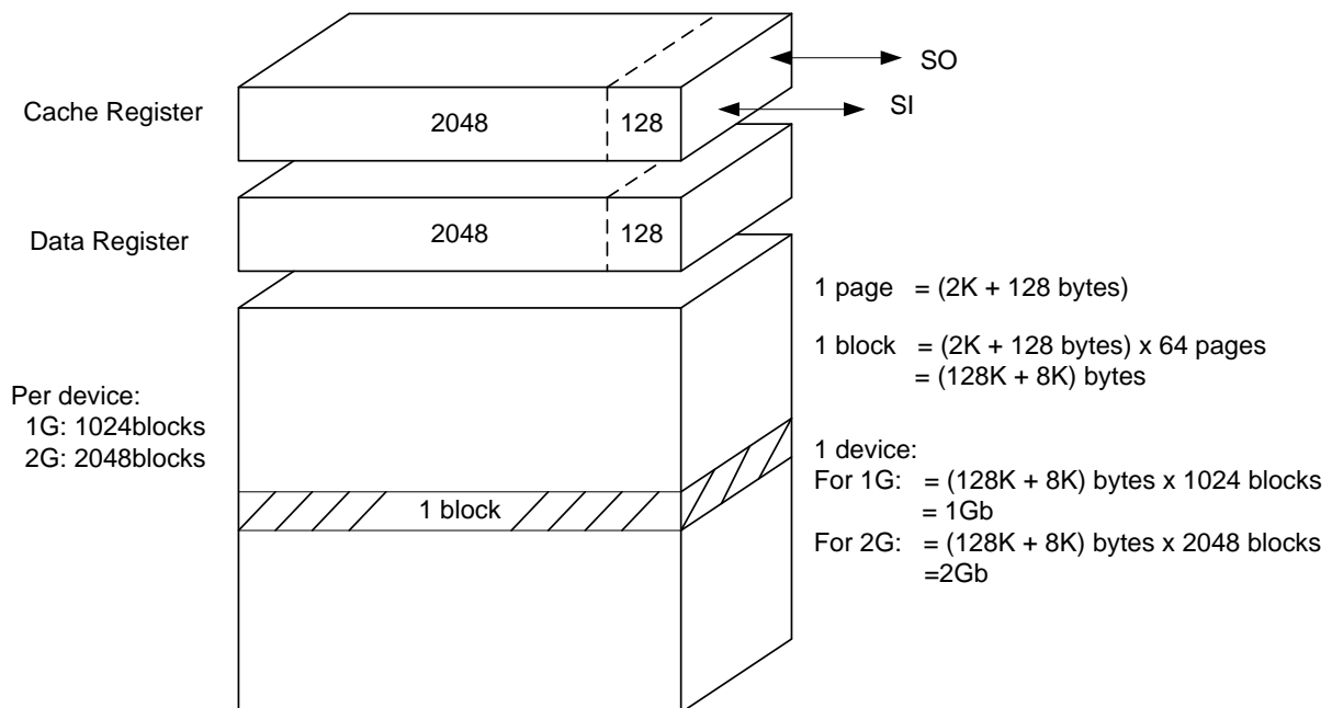
Figure1. Array Organization
