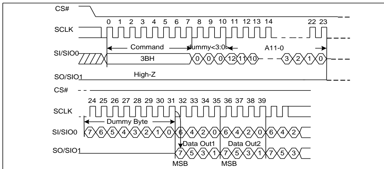
Figure10. Read From Cache x2 Sequence Diagram
