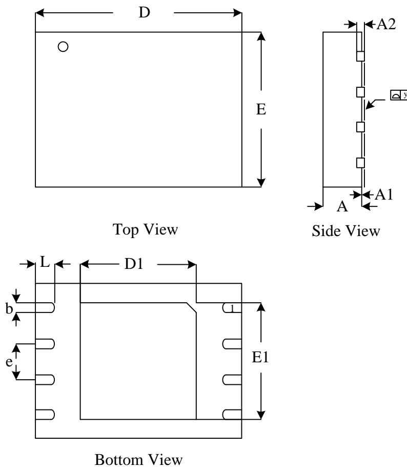
Figure29. WSON8 (8*6mm)
