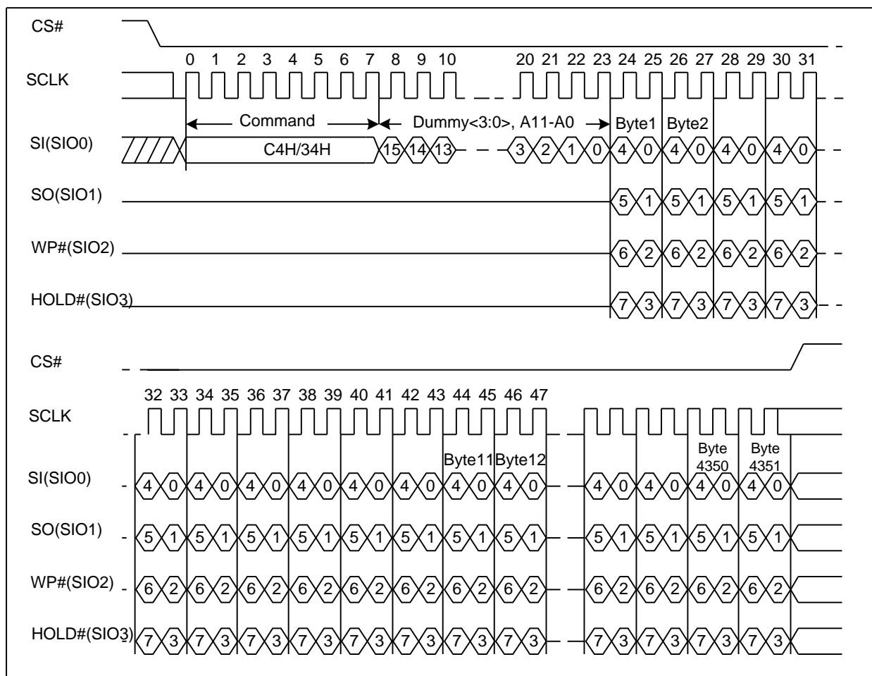
Figure19. Program Load Random Data x4 Sequence Diagram
